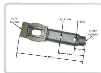
DA Pt # DA-41931 Alt Pt # DA-402-1 Description: Capstan, Long
