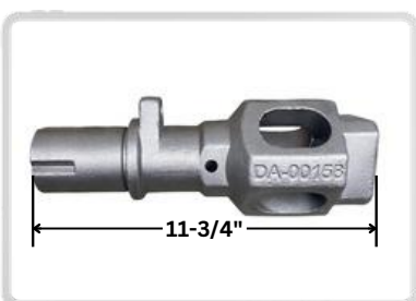
DA Pt # DA-00158 Alt Pt # 530-0158 Description: Capstan Casting
