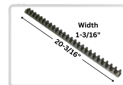
DA Pt # DA-70213 Alt Pt # 70213 Description: Rack 20-3/16" L x 1-3/16"W
