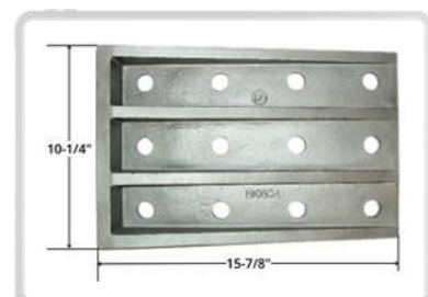
DA Pt # DA-18004 Alt Pt # B-10804 Description: Draft Lug, Rear
