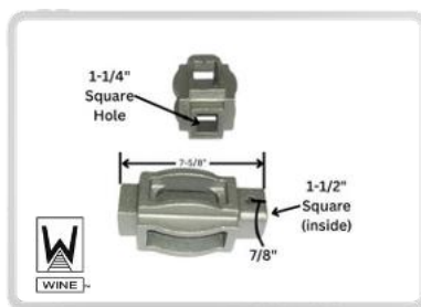
DA Pt # DA-01211 Alt Pt # 2CH-121 Description: Capstan - Outlet Gate
