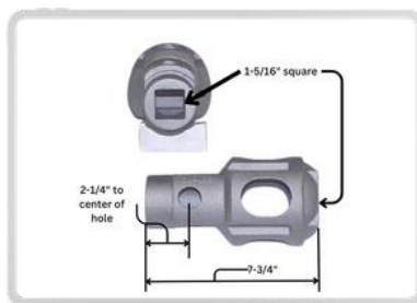
DA Pt # DA-42391 Alt Pt # DA-4081 Description: Capstan
