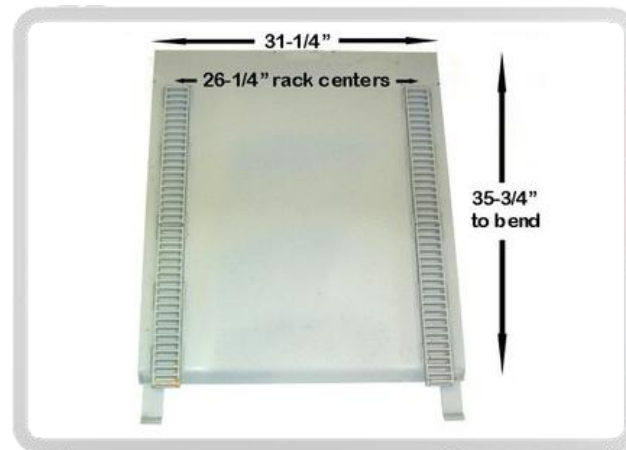
DA Pt # DA-50289 Alt Pt # 810-456723-0 Description: Door Slide Assembly
