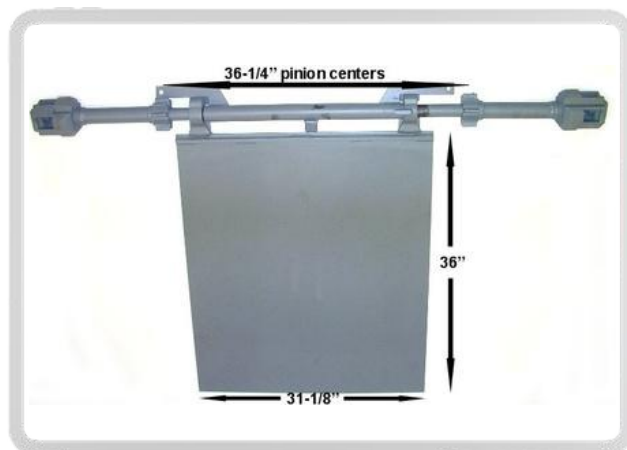
DA Pt # DA-71131 Alt Pt # 71131 Description: Door Slide Assembly
