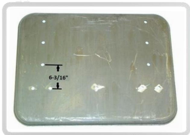
DA Pt # DA-176003-H Alt Pt # 176003H Description: Hopper Door w/ Spreader Beam Holes, Small, Carbon Steel, 5/16" Thick
