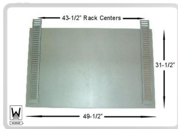
DA Pt # DA-41328 Alt Pt # 41328 Description: Door Slide Assembly
