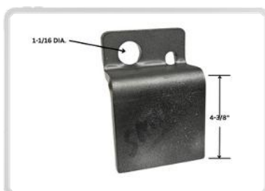
DA Pt # DA-28275-B Alt Pt # 28275 Description: Gate Lock Bracket
