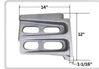
DA Pt # DA-15154 Alt Pt # 50154-R Description: Draft Lug, Rear, RH
