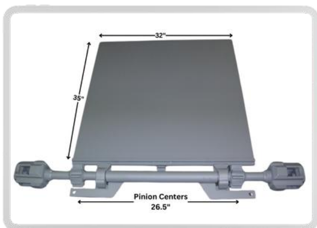
DA Pt # DA-71133 Alt Pt # 71133 Description: Door Slide Assembly
