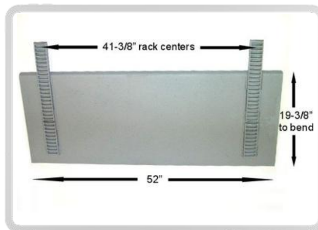
DA Pt # DA-50210 Alt Pt # 50210 Description: Door Slide Assembly
