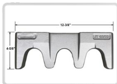
DA Pt # DA-09462 Alt Pt # 09462 Description: Draft Lug, Front, Forging
