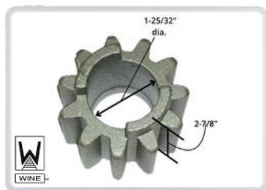
DA Pt # DA-21129 Alt Pt # CH-29 Description: Pinion Gear, 1-25/32" dia. Hole
