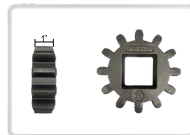
DA Pt # DA-70214 Alt Pt # 70214 Description: Pinion Gear, 1" Wide
