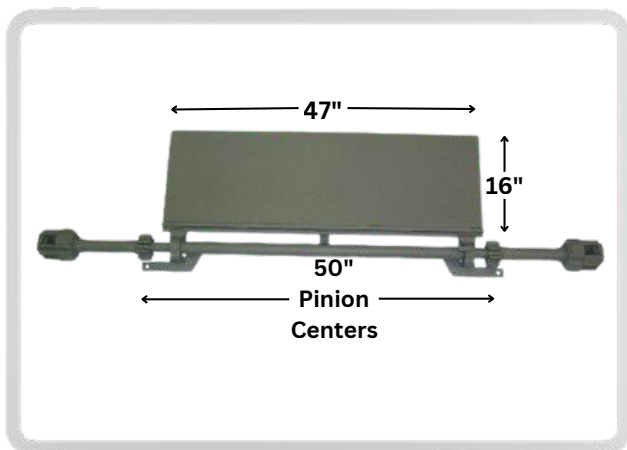
DA Pt # DA-71106 Alt Pt # 3000280 Description: Door Slide Assembly
