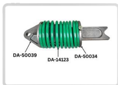
DA Pt # DA-50002-G Alt Pt # 50002G Description: Compressed Spring Assist Assembly #2
