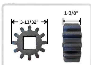
DA Pt # DA-70211 Alt Pt # 70211 Description: Pinion Gear, Square Hole, 1-3/8" W
