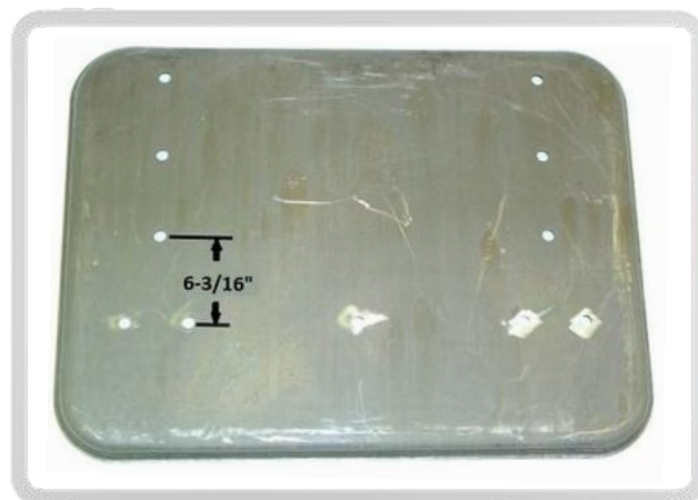
DA Pt # DA-76005-H Alt Pt # 76005H Description: Small, Carbon Steel 3/8" Thick w/ Spreader Holes
