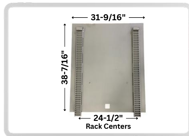
DA Pt # DA-10061 Alt Pt # 3000823 Description: Door Slide Assembly
