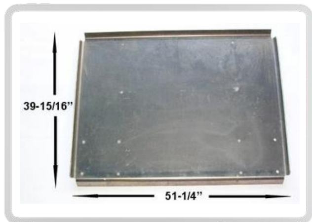
DA Pt # DA-17060 Alt Pt # 1020335 Description: Aluminum Hopper Door
