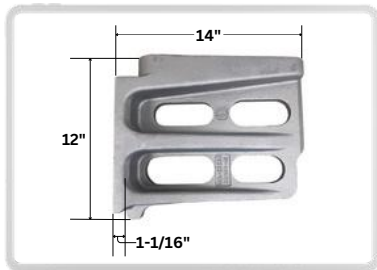
DA Pt # DA-15155 Alt Pt # 50154-L Description: Draft Lug, Rear, LH
