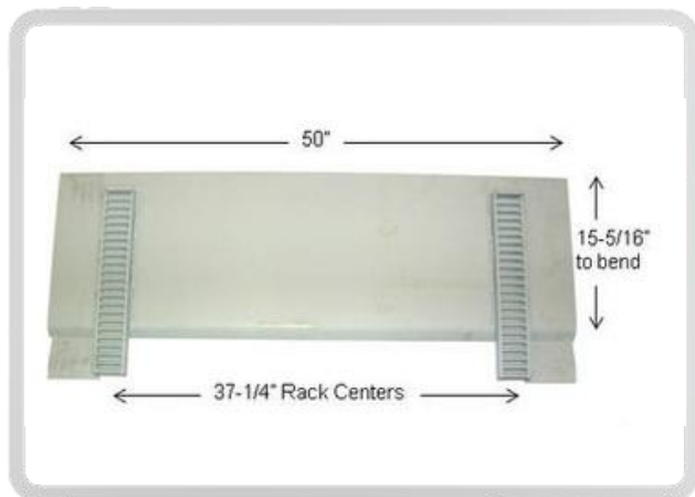
DA Pt # DA-11286 Alt Pt # 3000904 Description: Door Slide Assembly
