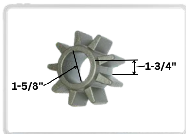
DA Pt # DA-69400 Alt Pt # OVPA-694 Description: Pinion Gear, 1-3/4" W x 1-5/8" dia.
