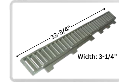
DA Pt # DA-42382 Alt Pt # VPA-6182 Description: Rack 33-3/4" L x 3-1/4" W
