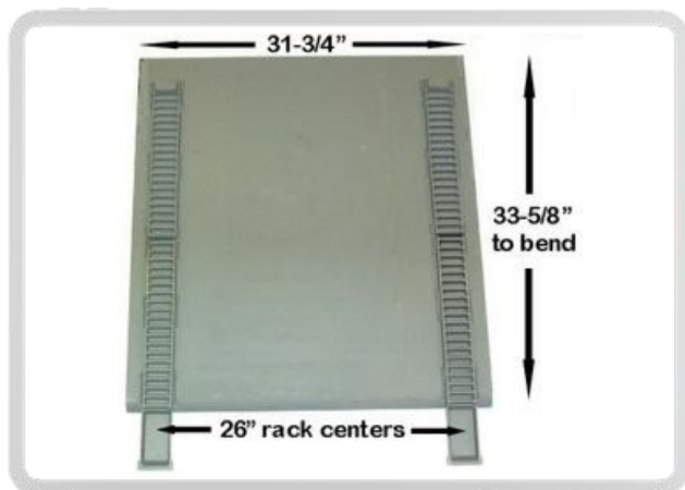
DA Pt # DA-78134 Alt Pt # 3000597 Description: Door Slide Assembly
