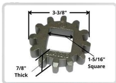
DA Pt # DA-70212 Alt Pt # 70212 Description: Pinion Gear
