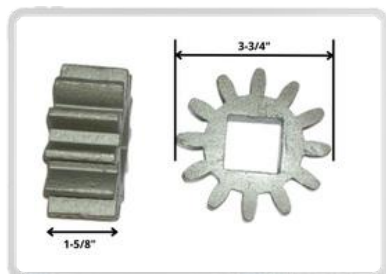
DA Pt # DA-70210 Alt Pt # DA-29-B Description: Pinion Gear, Square Hole
