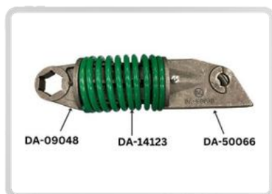
DA Pt # DA-50000-G Alt Pt # 50000G Description: Compressed Spring Assist Assembly #1
