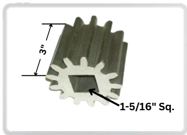
DA Pt # DA-30304 Alt Pt # DA-502-SS Description: Pinion Gear, Stainless Steel
